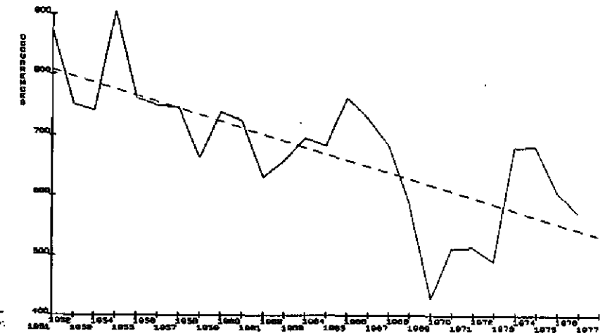
Figure 26. The annual frequency of middle clouds during 1951-1976 at Ft. Wayne, Springfield, St. Louis, and Evansville.
