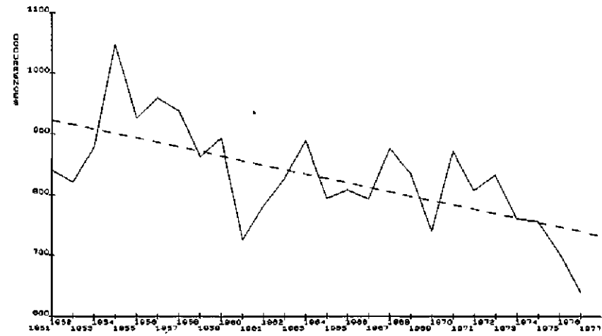
Figure 24. The annual frequency of middle clouds during 1951-1976 at Duluth, Sault Ste. Marie, Green Bay, and Madison.
